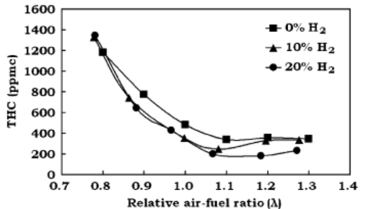
Fig. 7. Effect of H 2 addition on natural gas combustion hydrocarbon emissions [8]
