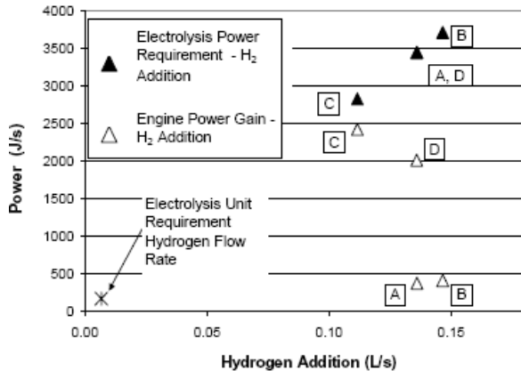
Fig. 11: The power requirement for electrolysis and the power gained from the engine through hydrogen addition (U of Windsor) [16]
