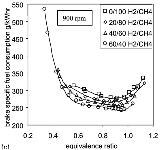
Fig. 5. Reduction in fuel consumption with increase in hydrogen addition [3]
