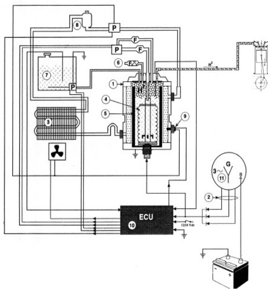
Fig. 1. General structure of the system (1. Electrolysis cell; 2. Secondary circuit; 3. Radiator; 4. Anode electrode; 5. Cathode electrode; 6. Air filter; 7. Water tank; 8. Cooling water tank; 9. Water temperature sensor; 10. Electronic control unit of the system; 11. Alternator. P – water pump, F – water filter).
