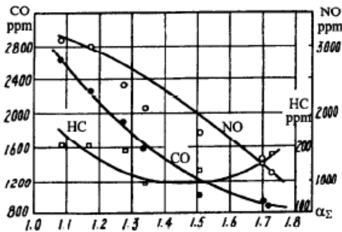
Fig. 9. Emission after hydrogen addition [2]
