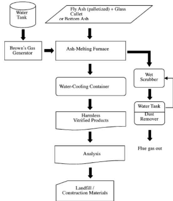
Fig. 15. Brown's Gas incinerator for vitrification of solid waste [20]
