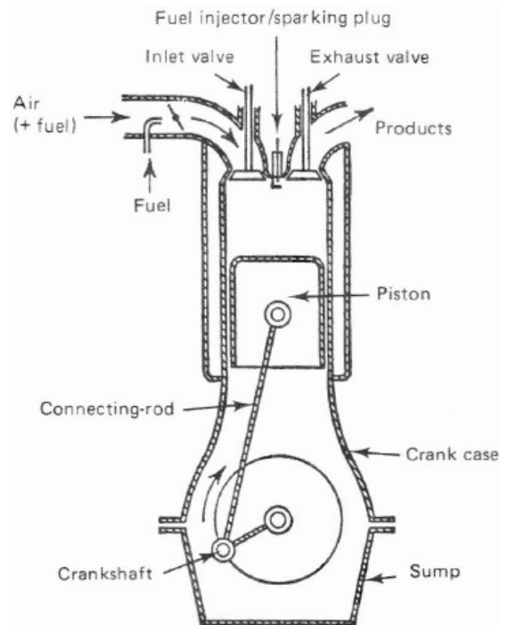
Fig. 1. Four Stroke Internal Combustion Engine [1]
