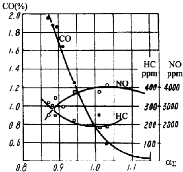
Fig. 2. Emission characteristics with gasoline fuel.
