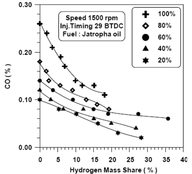
Fig. 6. Effect of H 2 addition on jatropha oil combustion CO emissions [6]
