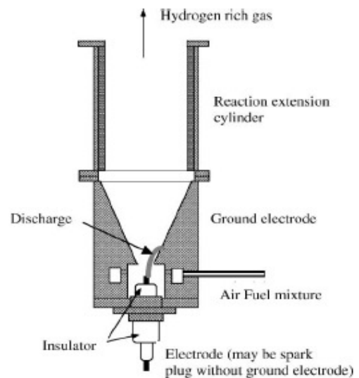
Fig. 10. Low current plasmatron fuel reformer [14]
