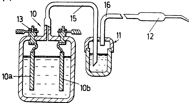
Fig. 13. Yull Brown's electrolysis unit from US Patent: 4,081,656 [18]
