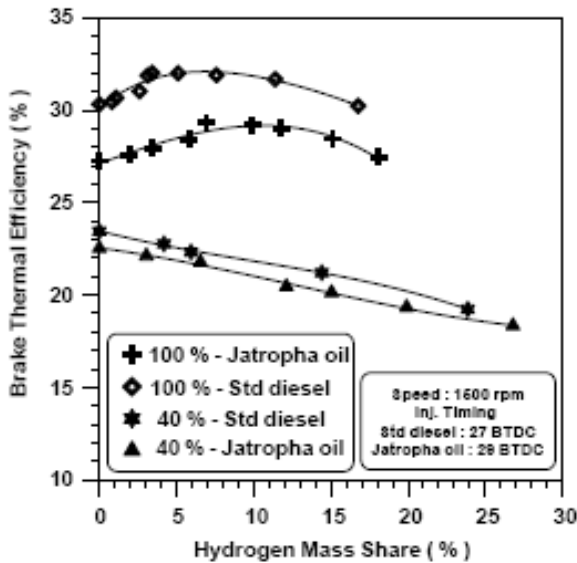
Fig. 4. Variation of thermal efficiency with hydrogen mass share [6]
